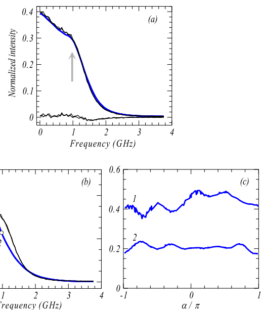
FIG. 2. Measured light scattering spectrum of Ar compared to MD simulations. (a) Using periodic boundary conditions and (b) with reflective boundary conditions. The full black lines are the experimental results, with positive and negative frequencies overlaid. The blue lines are the MD results. The lower black lines are the difference between experiments and MD results. All spectra were normalized to \int E(f) df = 1 , where the integration runs over one free spectral range. In (a), the arrow points to the frequency of sound with wavelength equal to the box size, and in (b), the arrow points to the sound frequency with wavelength equal to the twice the box size. Notice that due to the periodic instrument function, the high-frequency tails of the spectra do not return to E(f) = 0 exactly. (c) Dependence of the spectrum S(k_{\text{sc}}, \omega) on the angle \alpha with the x -axis of k_{\text{sc}} in the x y -plane. The random vectors were restricted to this plane, k_{\text{sc}_z}/k_{\text{sc}} < 0.1 . The two curves with 1, 2 correspond to the frequencies indicated in (b).
