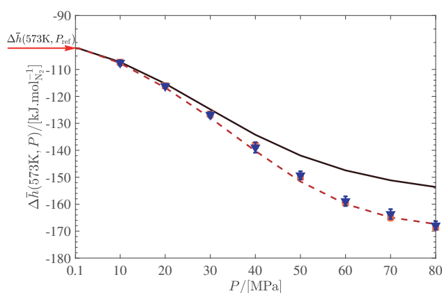
Figure 6. Computed reaction enthalpy of the Haber–Bosch process per mole of N 2 at 573 K and pressure range of P = 10\text{--}80 MPa. The arrow on the left indicates the value of the reaction enthalpy at standard reference pressure ( P_{ref} = 1 bar). The compositions of the mixtures are obtained from equilibrium simulations of the Haber–Bosch reaction using serial Rx/CFC [43]. Different methods used to compute enthalpy of reaction: PR EoS (solid line), PC-SAFT (dashed red line), ND method (squares), CFC/NPT ensemble (blue triangles). Zero BIPs were used for the EoS modelling. Raw data are listed in Table S12 of the Supporting Information (Online).
