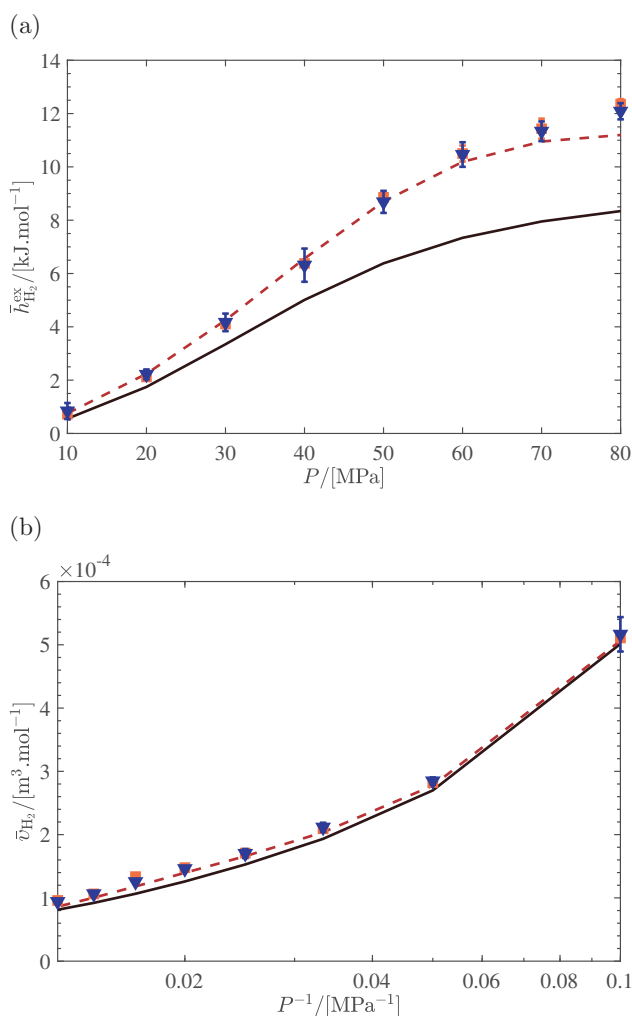
Figure 5. (a) Computed partial molar excess enthalpies of H 2 and (b) computed partial molar volumes of H 2 in a [NH 3 , N 2 , H 2 ] equilibrium mixture at 573 K and pressure range of P = 10\text{--}80 MPa. The compositions of the mixtures are obtained from equilibrium simulations of the Haber–Bosch reaction using serial Rx/CFC [43], and are listed in Table S1 of the Supporting Information (Online). In both subfigures: computed properties using the PR EoS (solid black line), computed properties using the PC-SAFT (dashed red line), computed properties using the ND method (squares), computed properties in the CFC/NPT ensemble (triangles) using Equations (8) and (9). Zero BIPs were used for the EoS modelling. Raw data are listed in Table S6 of the Supporting Information (Online).
